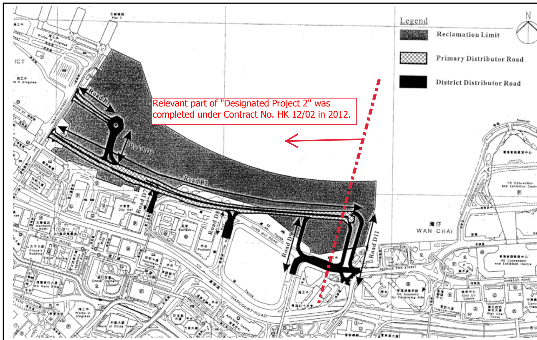
Figure 2: Primary and District Distributor Roads- Layout Plan
