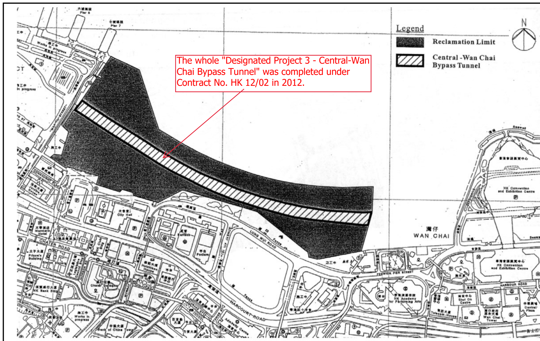
Figure 3: Central – Wan Chai Bypass Tunnel – Layout Plan
